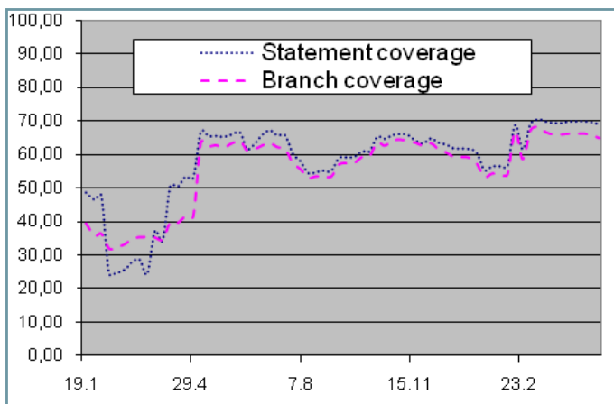
Figure 1: Coverage measurements to guide test improvements
